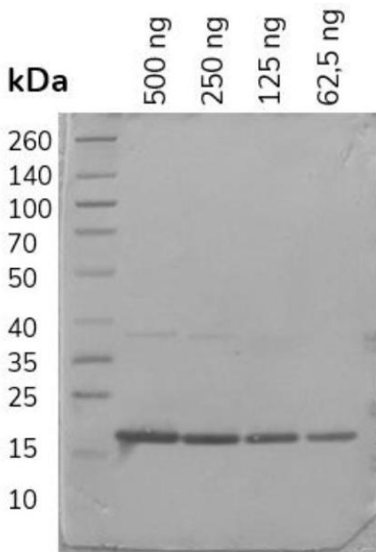
Figure 2. Western blot: decreasing amounts of TNF Alpha (17 kDa) detected with Human Anti-TNF Alpha (Biotin) at 1: 2 000 and HRP conjugated Streptavidin at 1: 5 000.
